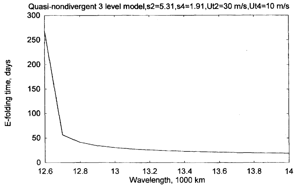
Fig. 23: The e-folding times in days for the three level quasi-nondivergent model for the longer waves.
