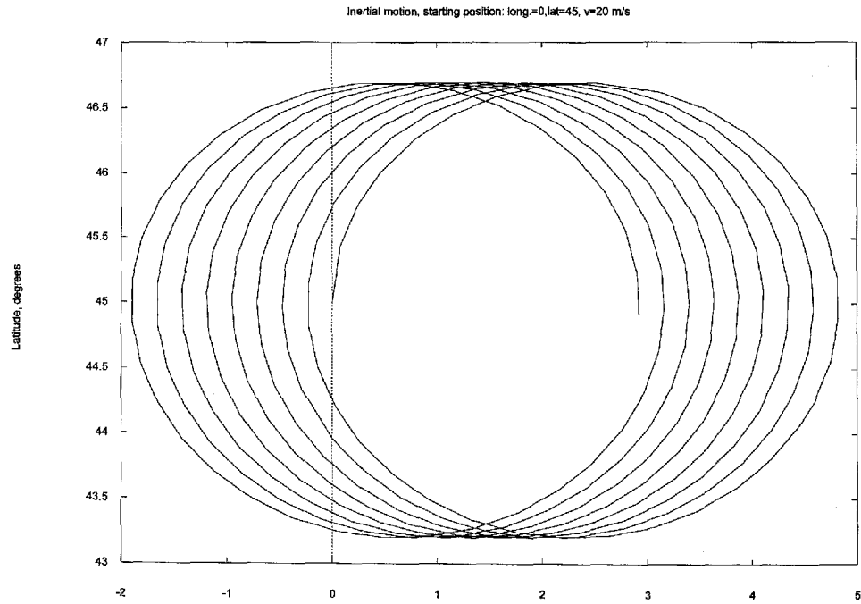
Fig. 27: Inertial motion starting from \lambda = 0 , \phi = 25 , v = 20 m per s.
