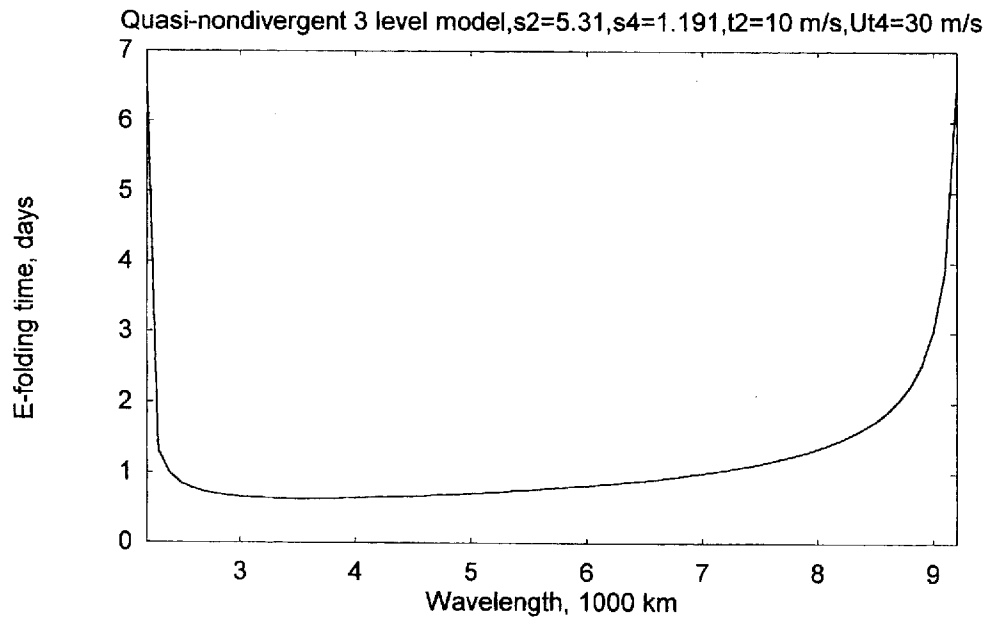
Fig. 24: As Figure 22, but with U_{T2} = 10 m per s and U_{T4} = 30 m per s.
