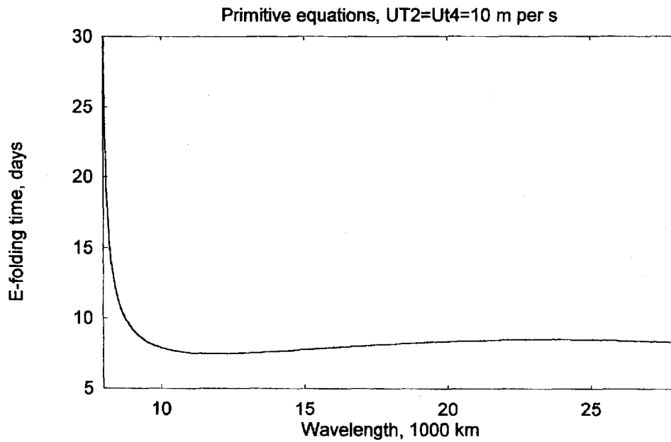
Fig. 17: As Figure 16, but for long waves.
