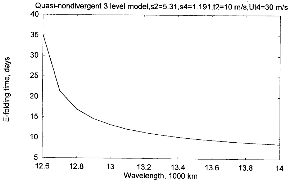
Fig. 25: As Figure 23, but with U_{T2} = 10 m per s and U_{T4} = 30 m per s.
