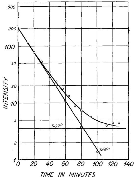
Fig. 7. Disintegration curve of radioactivity of \text{Rb}^{91} 14^m after chemical separation of Sr. The curve shows that the 9.7^h Sr is a daughter substance of this isomer.
