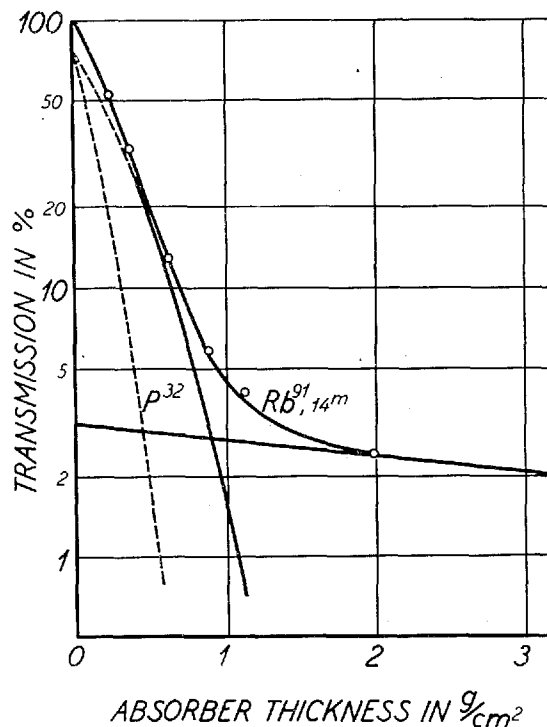
Fig. 10. Absorption curve for \text{Rb}^{91} 14^m obtained after chemical separation of Sr. E^{\text{max}} = 3.0 \text{ MeV} .
