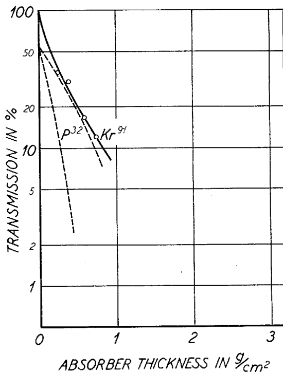
Fig. 12. Absorption curve for \text{Kr}^{91} . E^{\text{max}} = 3.6 \text{ MeV} .
