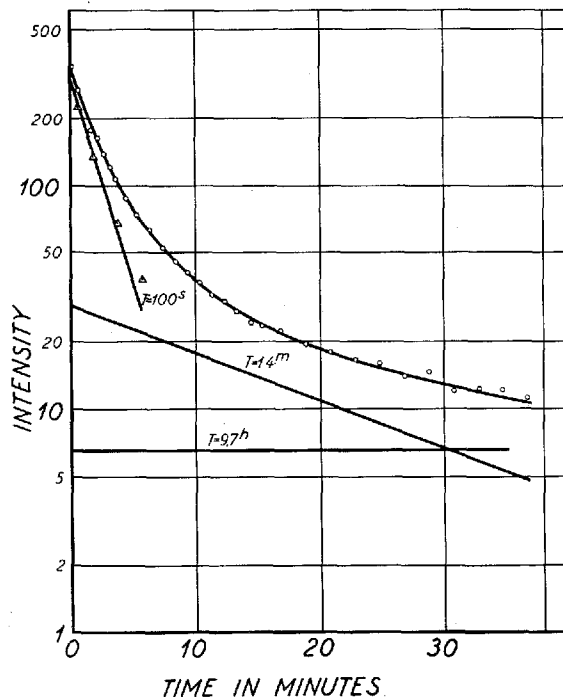
Fig. 8. Disintegration curve of radioactivity of Rb 91 100 s , Rb 91 14 m and Sr 91 including the growth of the 50 m isomer of Y 91 . Although the procedure is not exact we have chosen to subtract the effect of Sr 91 and Y 91 as a constant.
