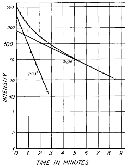
Fig. 4. Disintegration curve of radioactivity of Kr^{90} and its daughter Rb^{90} .
