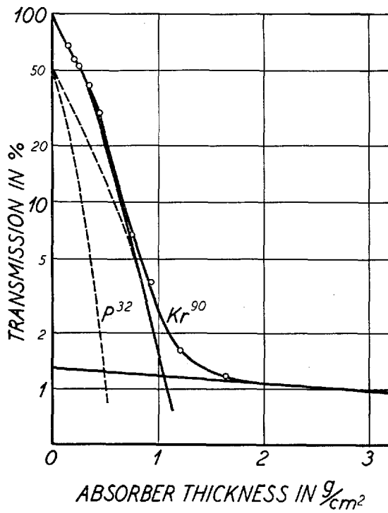
Fig. 6. Absorption curve for Kr^{90} . E_{max} = 3.2 MeV.
