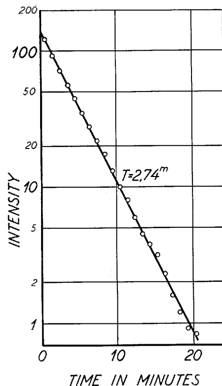
Fig. 3. Disintegration curve of radioactivity of Rb 90 . The zero counting rate and a small amount of 15.4 m Rb 89 activity due to KrH ions has been subtracted.
