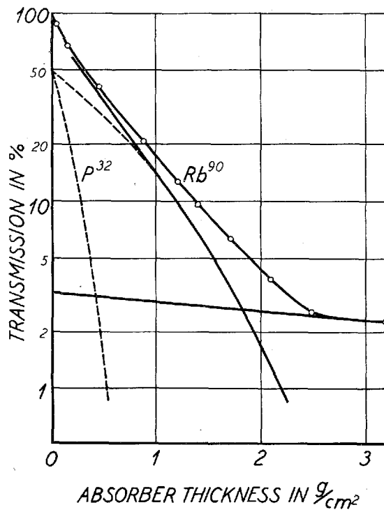
Fig. 5. Absorption curve for Rb^{90} . E_{max} = 5.7 MeV.
