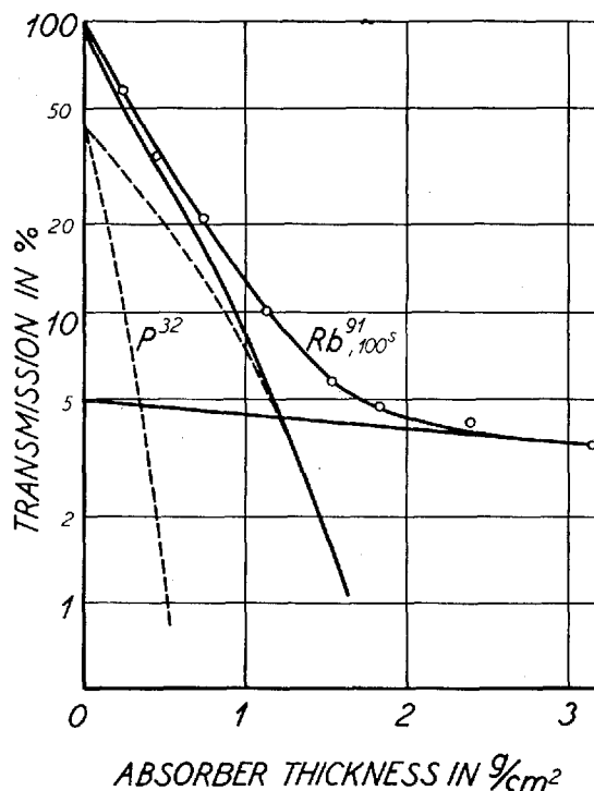
Fig. 11. Absorption curve for \text{Rb}^{91}, 100^s . E^{\text{max}} = 4.6 \text{ MeV} .
