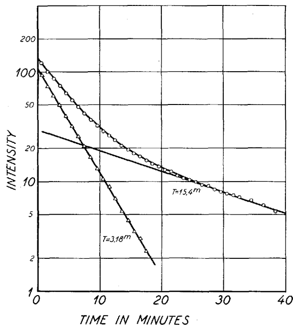
Fig. 1. Disintegration curve of radioactivity of mass number 89.
