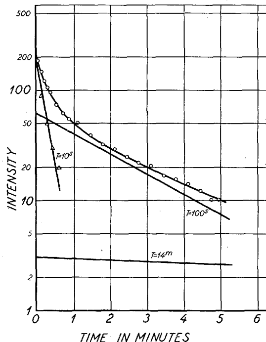
Fig. 9. Disintegration curve of radioactivity of Kr 91 10 s and its daughter substances Rb 91 100 s and Rb 91 14 m .
