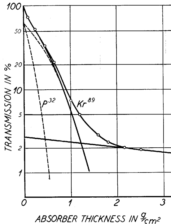
Fig. 2. Absorption curve for Kr^{89} . E^{max} = 4.0 MeV.
