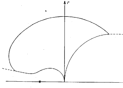
Fig. 5. The boundary curve of an asymmetrical spectrograph ( z_{f1} \neq z_{f2} ) with b = 1 and with a symmetrical arrangement of orbits ( \zeta(a) = 0 ).
