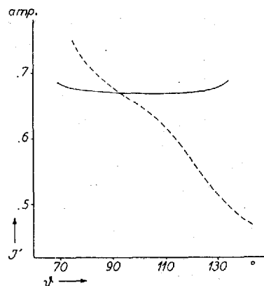
Fig. 10. The current, J' , in the electromagnet corresponding to focusing of the ThBF -line, as a function of the direction of emission of the \beta -rays, \theta . The dotted and the full-drawn lines, respectively, correspond to the uncorrected and the corrected pole pieces.
