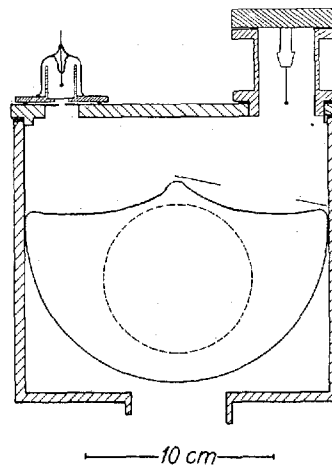
Fig. 9. A section parallel to the axis of the 30^\circ model showing source, focus and one of the pole pieces.
