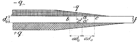
Fig. 64. Sketch of Distribution of Charge at the Edge of a Negative Figure.
