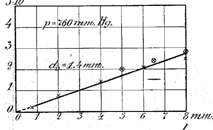
Fig. 51. Relation between Velocity U and Spark Length l for Negative Figures. (Air; p = 760 ; d_0 = 1.4 ).
