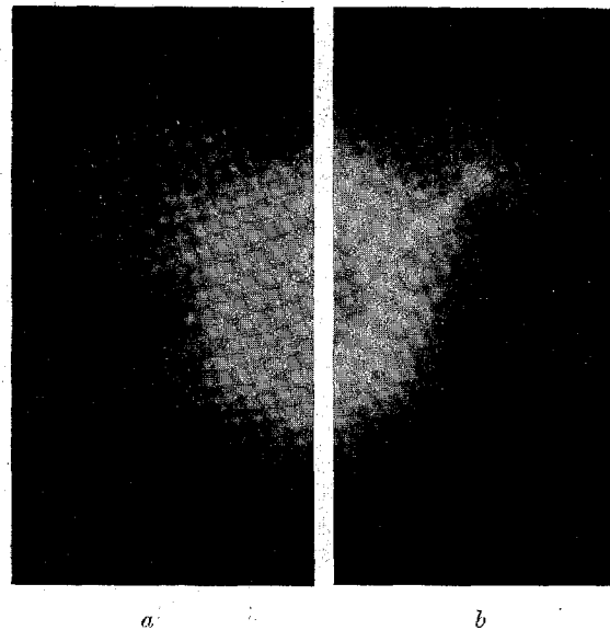
Fig. 24. a Lower and b Upper Tertiary Figure for Negative Discharge. (Air; p = 760 ; l = 8 ; D = 17.5 ; d_s = 0.1 ; m = 1 ).
