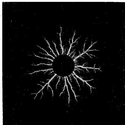
Fig. 30. Oscillating Discharge, first Half-wave Positive. L = 133 cm. (Air: p = 760 ; l = 10 ; D = 9.5 ; d_0 = 1.3 ; m = 1 ).
