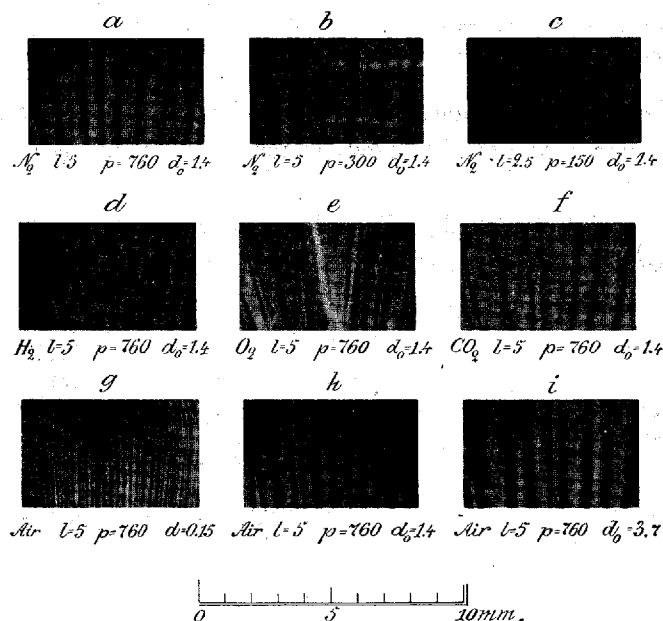
Fig. 32. Parts of Negative Figures in various Gases and at various Pressures.
