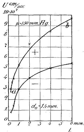
Fig. 57. Effect of Spark Length on the Positive and Negative Velocity. (Air; p = 150 ; d_0 = 1.4 ).
