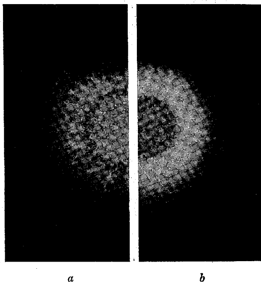
Fig. 23. a Lower and b Upper Tertiary Figure for Negative Discharge. (Air; p = 760 ; l = 8 ; D = 17.5 ; d_s = 0.1 ; m = 1 ).
