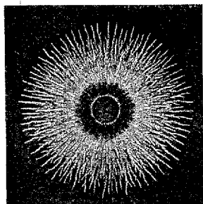
Fig. 2. Positive Lichtenberg Dust Figure. (Air; p = 760 ; m = 0.8^* )
