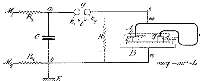
Fig. 43. Circuit Connections in Velocity Measurements.
