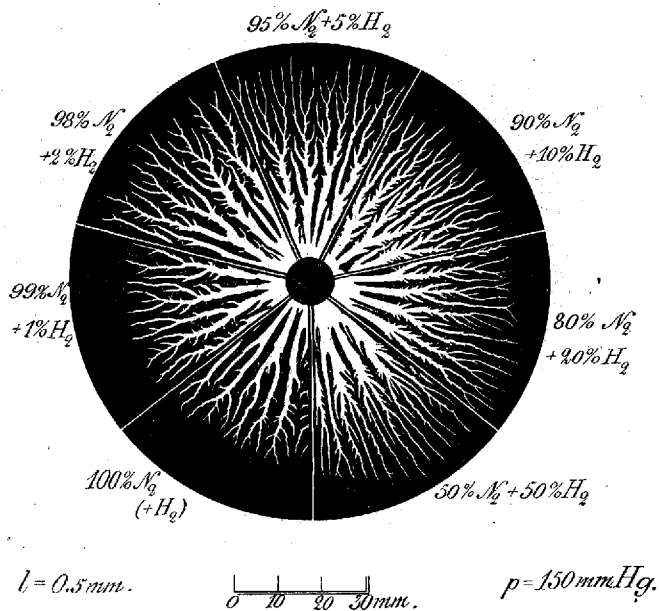
Fig. 70. Sections of Positive Figures in Mixtures of Nitrogen and Hydrogen.
