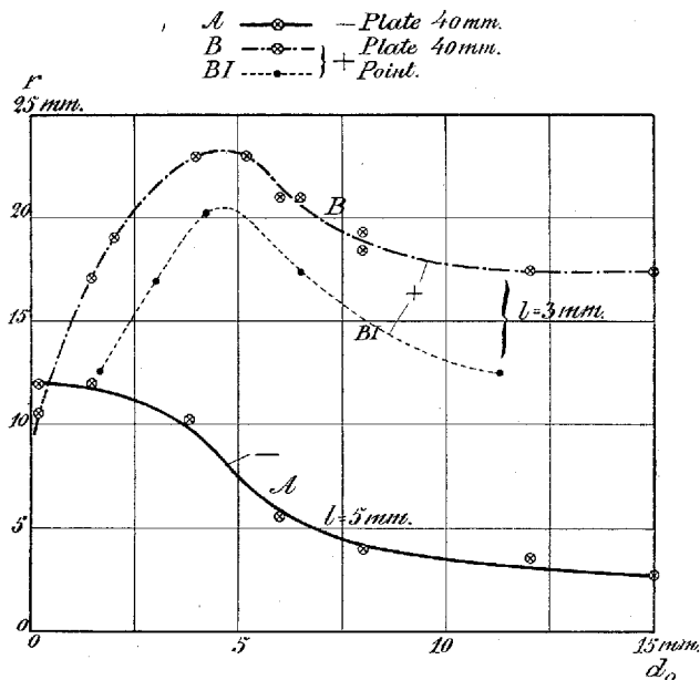
Fig. 34. Relation between Range and Thickness of Plate for Photographic Figures.
