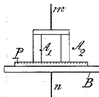
Fig. 11. Lichtenberg Figures from several Parallel Electrodes.
