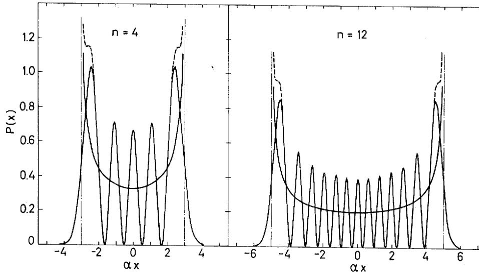
Fig. III.1: Spatial density for harmonic-oscillator eigenfunctions corresponding to n = 4 and n = 12 , respectively. The classical turning points are indicated by dot-and-dash lines, and the classical spatial probability (Eq. (III.9)) is given by the smooth solid curve. The oscillating solid curve corresponds to the exact distribution |u_n(x)|^2 (Eq. (III.7)) and the dashed curve to the density obtained from the WKB approximation (Eq. (III.22)).
