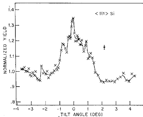
Fig. I.12: Scan through \langle 111 \rangle axis for the 2.8\text{-}\mu\text{m} sample. The error flag on the upper right-hand side indicates beam divergence and statistical uncertainty of the measurements.
