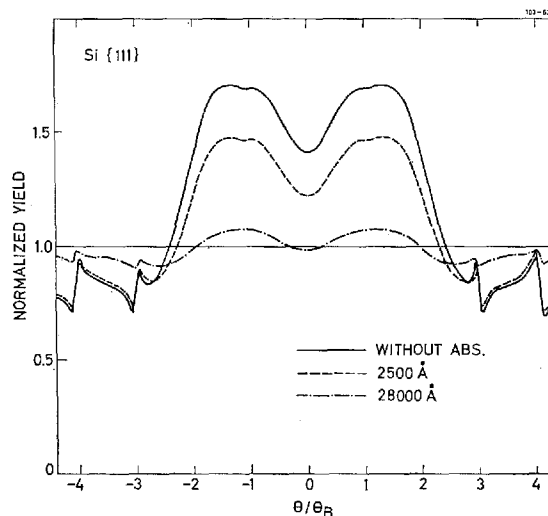
Fig. II.5: 20-beam planar calculation for e^- on Si. Effects of thermal vibration are included according to Eqs. (II.15) and (II.17), and the influence of incoherent scattering has been estimated as described for the previous figure.
