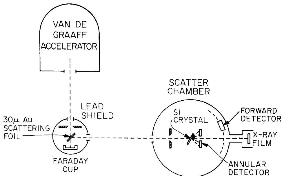
Fig. I.1: Experimental arrangement.
