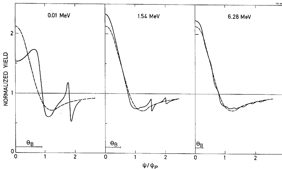
Fig. IV.4: Comparison of classical and quantal calculations of the peak in large-angle-scattering yield for electrons incident on Si along a \{110\} plane. The classical yield is derived from formulas analogous to those given in Ref. 29 for positive particles, with a thermally averaged Molière planar potential 41 , including the contributions from the neighbouring plane (cf. Fig. IV.1). The quantal result is obtained from a 20-beam calculation (Eq. (II.23)), also with the Molière potential and including effects of thermal vibrations (Eqs. (II.15) and (II.17)). The classical result scales with the planar characteristic angle \psi_P = \psi_1(Ca/d)^{1/2} , where d is defined through Nd^2dp = 1 (Ref. 29). For each projectile energy, the magnitude of the Bragg angle \theta_B is indicated (classical calculations: dashed curves; quantal calculations: solid curves).
