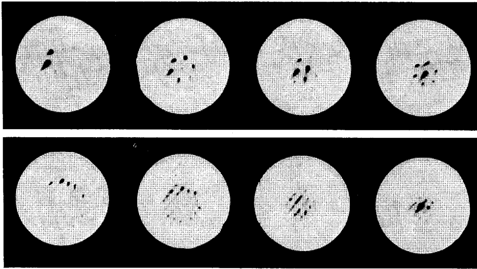
Fig. I.8: Film exposures of the forward beam for the 0.2–0.3 \mu\text{m} sample. The upper series corresponds to incidence angles of 0.6°, 0.4°, 0.2°, and 0°, relative to a \langle 111 \rangle axis, the lower series to incidence angles of 0.75°, 0.50°, 0.25°, and 0°, relative to a \langle 110 \rangle axis.
