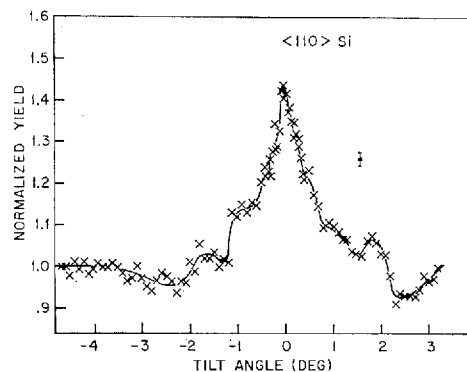
Fig. I.13: Scan through \langle 110 \rangle axis for the 2.8\text{-}\mu\text{m} sample. The error flag on the upper right-hand side indicates beam divergence and statistical uncertainty of the measurements.
