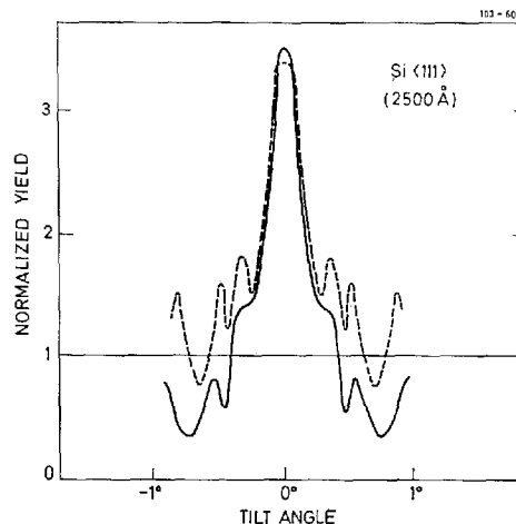
Fig. II.4: Axial peak in large-angle scattering yield for 0.7-MeV e^- , derived from a 49-beam calculation (cf. Fig. II.3). The influence of incoherent scattering has been estimated by including an imaginary component in the potential and assuming scattering into plane-wave states. The magnitude of the imaginary Fourier components of the potential has been evaluated from an approximation to the results given in Ref. 38. The peak derived from this calculation is compared to that obtained without absorption, multiplied by 0.5, corresponding to the correction for inelastic scattering applied in Figs. I.6 and I.7 (dashed curve).
