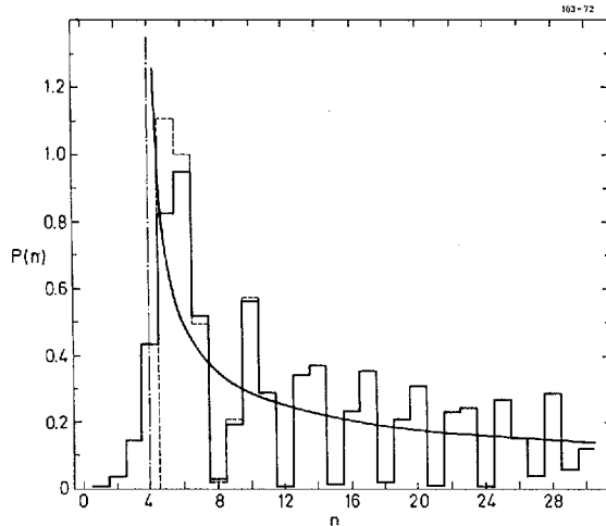
Fig. III.3: Population of levels in harmonic oscillator for \psi(x, t=0) = \exp(ikx) , with a value of k corresponding to (\hbar k)^2/(2M) = 4.5 \hbar\omega . This lower limit for the classical energy population is indicated by a dot-and-dash line, and the classical distribution (Eq.(III.10)) is given by the smooth solid curve. The solid staircase distribution corresponds to the exact population (Eq. (III.14) divided by \hbar\omega ), while the result obtained from the WKB approximation (Eq. (III.35)) is indicated by the dashed lines. Normalization and notation as for Fig. III.2.
