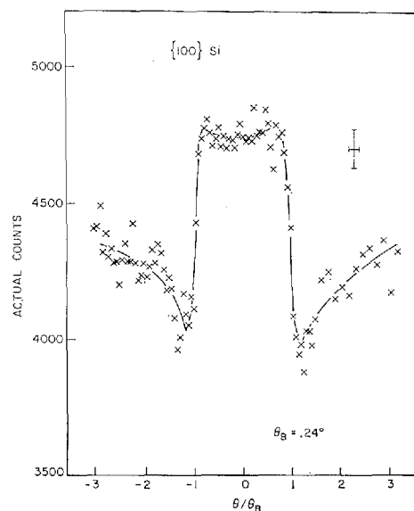
Fig. I.11: Scan through \{100\} plane for the 2.8\text{-}\mu\text{m} sample. The error flag on the upper right-hand side indicates beam divergence and statistical uncertainty of the measurements.
