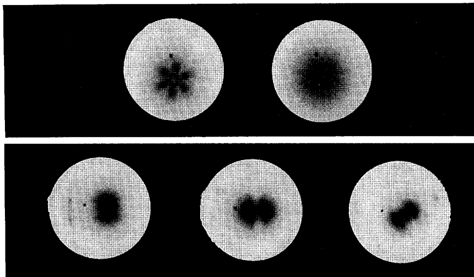
Fig. I.14: Film exposures of the beam transmitted through the 2.8\text{ }\mu\text{m} crystal. The upper two exposures correspond to beam incidence parallel to a \langle 111 \rangle axis and a \langle 110 \rangle axis. The lower three exposures correspond to incidence along \{100\} , \{110\} , and \{111\} planes. The small intense spot visible in all exposure is due to x rays produced in the gold scattering foil.
