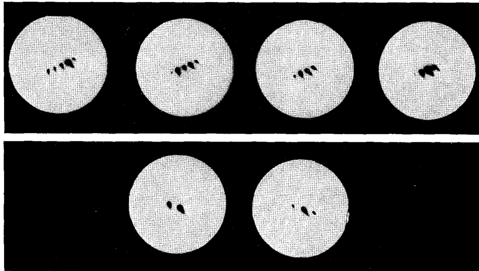
Fig. I.5: Film exposures of the forward beam for the 0.2\text{--}0.3\text{ }\mu\text{m} sample. The upper series of four exposures corresponds to the incidence angles of 3\theta_B , 2\theta_B , and \theta_B , and 0 with respect to a \{111\} plane. The lower two exposures correspond to incidence angles of \theta_B and 0 with respect to a \{110\} plane.
