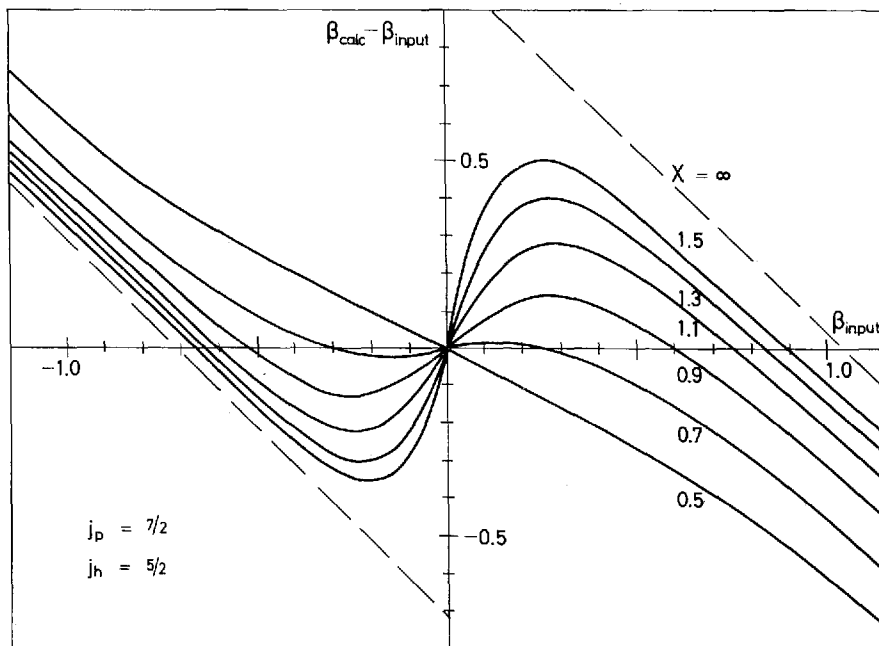
Fig. 6. Illustration showing the instability of a spherical 2p-2h excitation with respect to deformation. Details are explained in the text.
