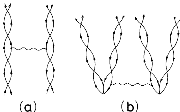
Fig. 5. Typical diagrams in the conventional fermion representation which contribute to the term H_{ph} decomposed in fig. 4. The diagram (a) occurs, for example, in \mathfrak{S}_{ph} , and (b), for example, in \mathfrak{S}_V .
