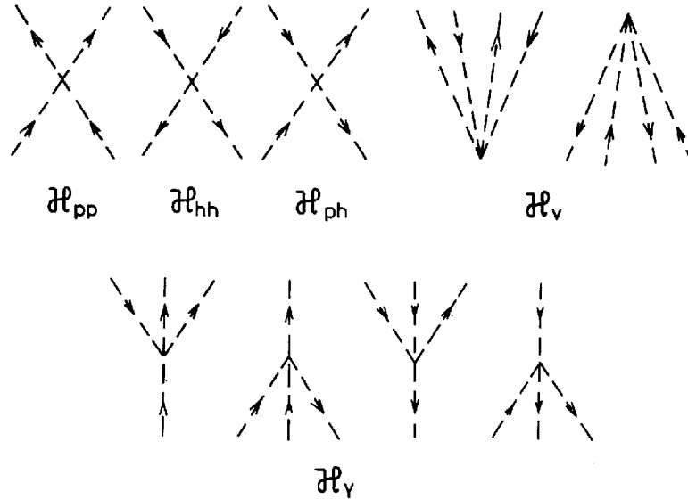
Fig. 4. Graphic representation of the matrix elements arising from the particle-hole interaction or the field-producing force. The broken lines indicate pair scattering modes, for a "particle pair" if the arrow points upwards, for a "hole pair", if the arrow points downwards.
