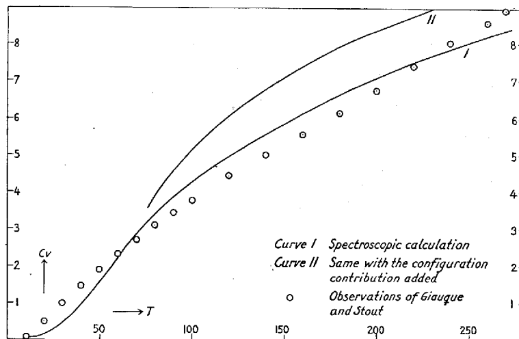
Fig. 5. Heat capacity of ice ( C_v ). Curve I: spectroscopic calculation. Curve II: Same with the configuration contribution added. \odot : Determinations of GIAUQUE and STOUT.
