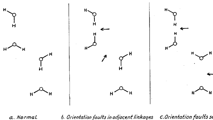
Fig. 3. Formation of orientation fault sites.
