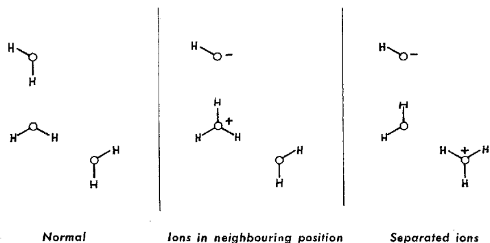
Fig. 1. Formation of ions by proton jumps.
