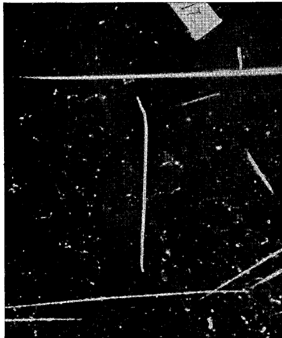
Fig. 5. Track of the long range group. Shows the characteristic bending in both ends.
