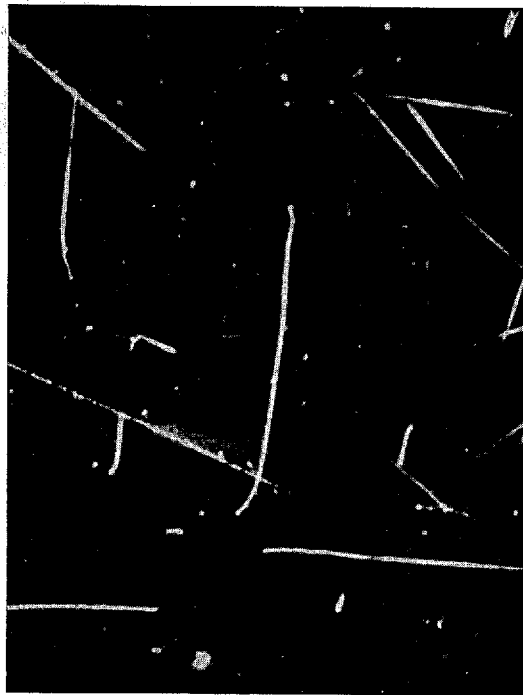
Fig. 3. Track of boron disintegration. The type of track is established by means of the characteristic feature, i. e., the fortuitous bending of both ends of the track demonstrates that the velocity is small in both ends. The track is thus produced by two ionizing particles originating somewhere in the track and moving in opposite directions.
