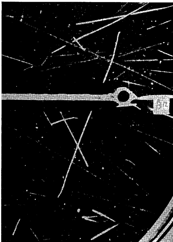
Fig. 9. Pared tracks of a boron disintegration. The boron is evaporated as a very thin layer ( 0.04 \text{ mg/cm}^2 ) on a gold leaf. The white band in the middle of the photo is the frame supporting the gold and boron foils. The short range Li-atom goes upwards and the He-atom downwards through the gold foil. It will be noticed that the tracks are not visible right up to their common point of origin, but that the foil on both sides is surrounded by a condensation-free space.
