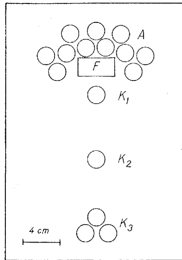
Fig. 1. Arrangement of counter tubes.
