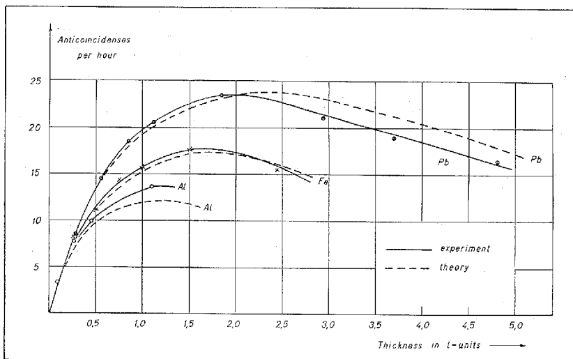
Fig. 2. Photon-initiated Rossi-Curves for Pb, Fe and Al.
