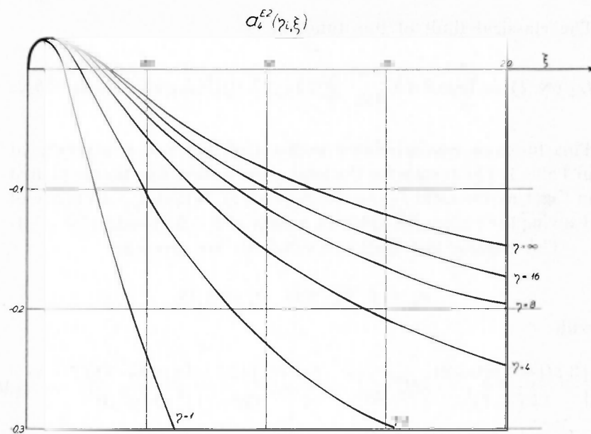
Fig. 3. The angular distribution coefficient a_4 as a function of \xi for different values of \eta_i .
