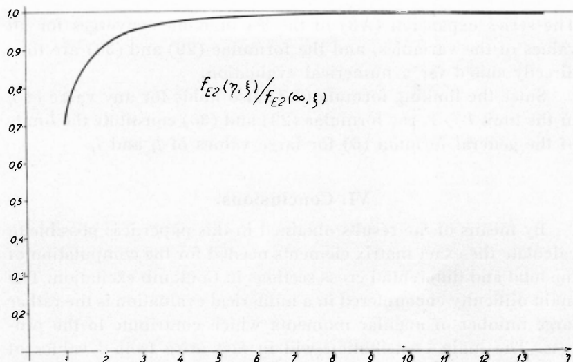
Fig. 1. The ratio of the exact to the classical total cross section function f_{E2}(\eta, \xi) / f_{E2}(\infty, \xi) for electric quadrupole excitation as a function of \eta . The curves for different values of \xi \leq 2 coincide within the accuracy of drawing for \eta > 1 .
