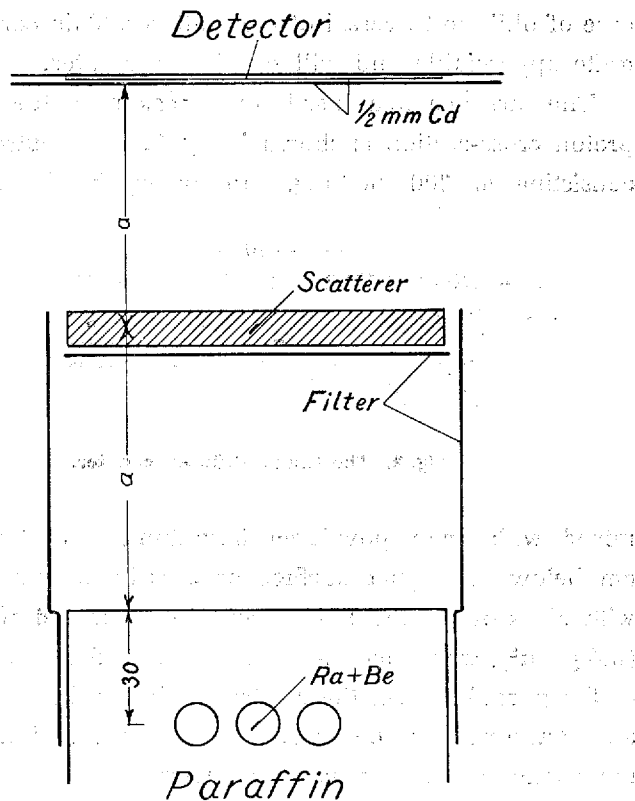
Fig. 1. Arrangement for neutron-proton scattering cross-section experiments.
