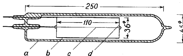
Fig. 2. The GEIGER-MÜLLER counter.
