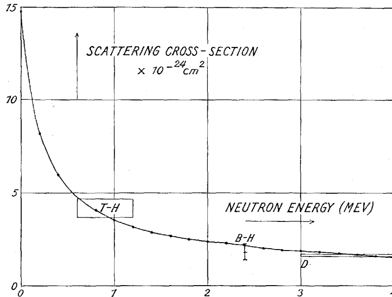
Fig. 4. Graph of WIGNER's formula.
